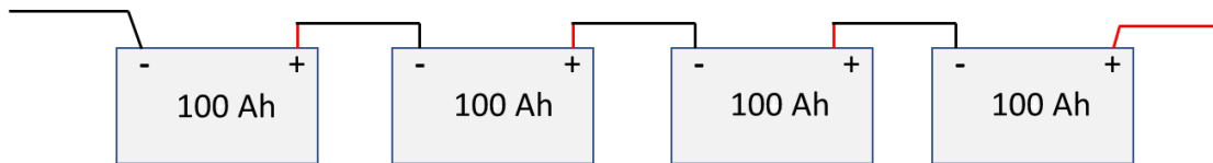
Series - 48 V 100 A Draw Capacity 90 Ah Capacity at 90%
