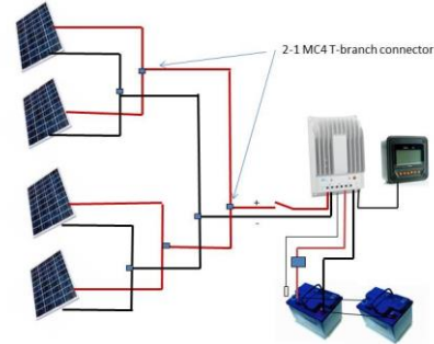
Four Solar Panels Wired in Parallel with One EP Tracer BN MPPT Controller
